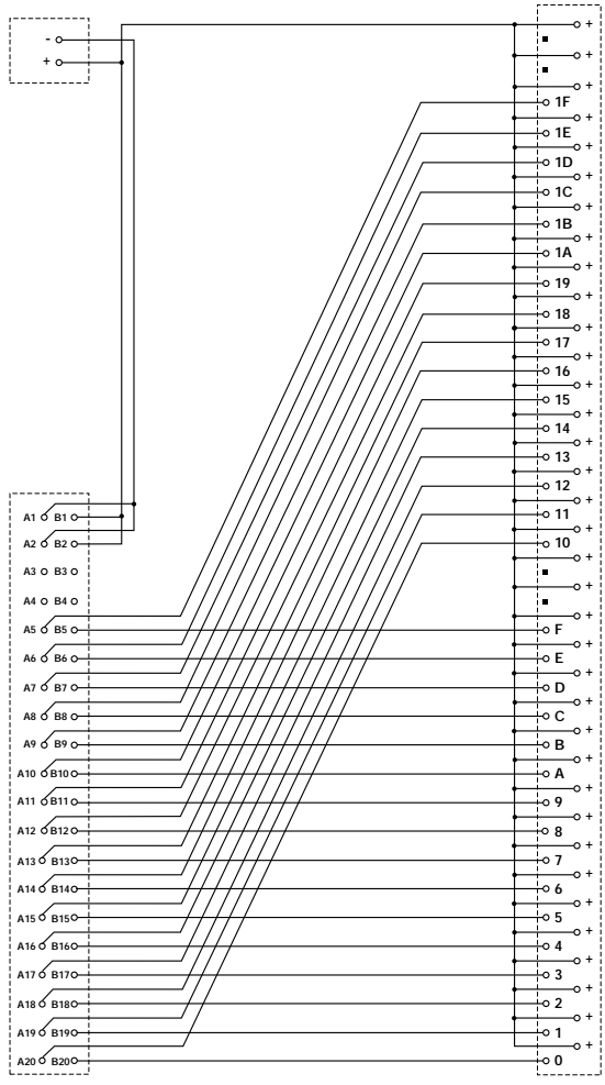
Passive - 2 wire 32 Channel Output Mitsubishi
