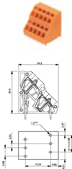
LM2NZF 5.08/135
