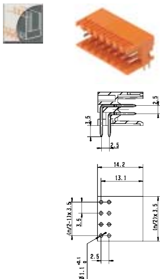
Pin headers S2L 3.5/90
