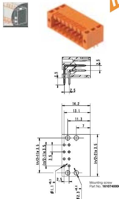
Pin headers S2L 3.5/90F
