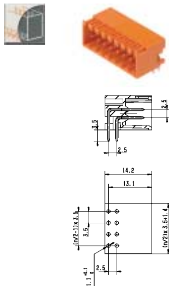
Pin headers S2L 3.5/90G
