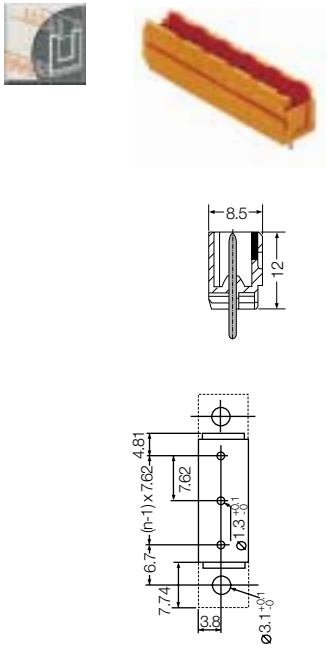
Pin headers SL 7.62/180B
