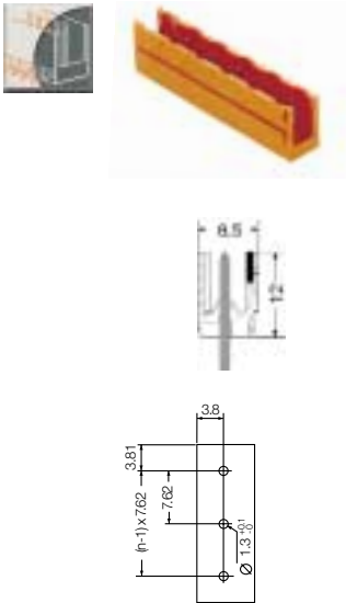
Pin headers SL 7.62/180
