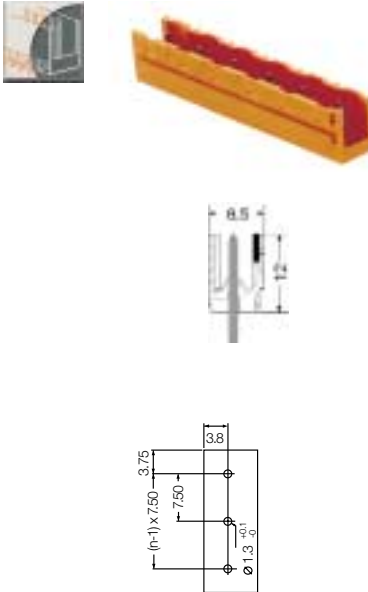
Pin headers SL 7.50/180
