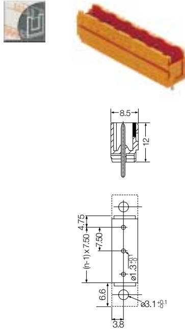
Pin headers SL 7.50/180B
