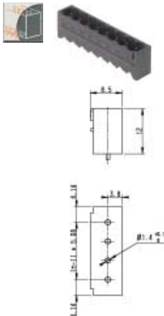
Pin headers SL-SMT 5.08/180G
