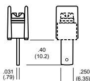
09 .250 QC w/o insulated base
