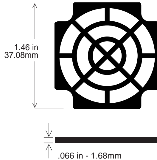
Retainer
