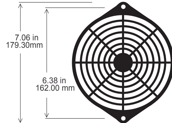
Guard
