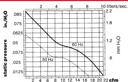
99XM Performance Curve
