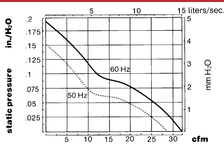
99XW Performance Curve
