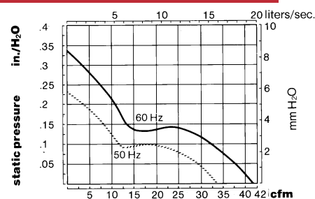
99XU Performance Curve
