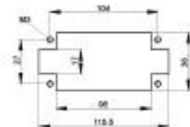
Panel Cut-Out
