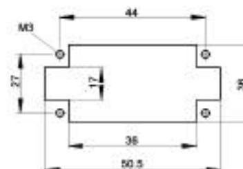
Panel Cut-Out
