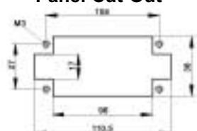
Panel Cut-Out
