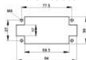
Panel Cut-Out
