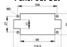
Panel Cut-Out
