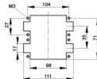
Panel Cut-Out
