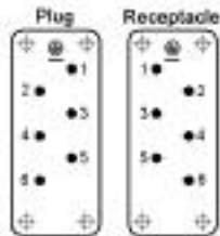
View from cable side
