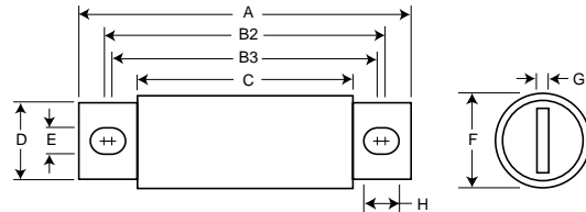
Fig. 2: 35-400 Amp Range
