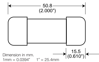
Fig. 1: 1-30 Amp Range
