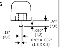
STYLE 6 Solder Turret
