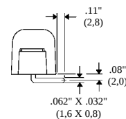
STYLE 8 Right Angle PC
