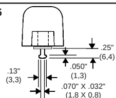
STYLE 6 Solder Turret
