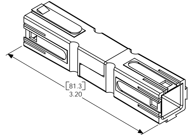
MATED PAIR OF HOUSINGS
