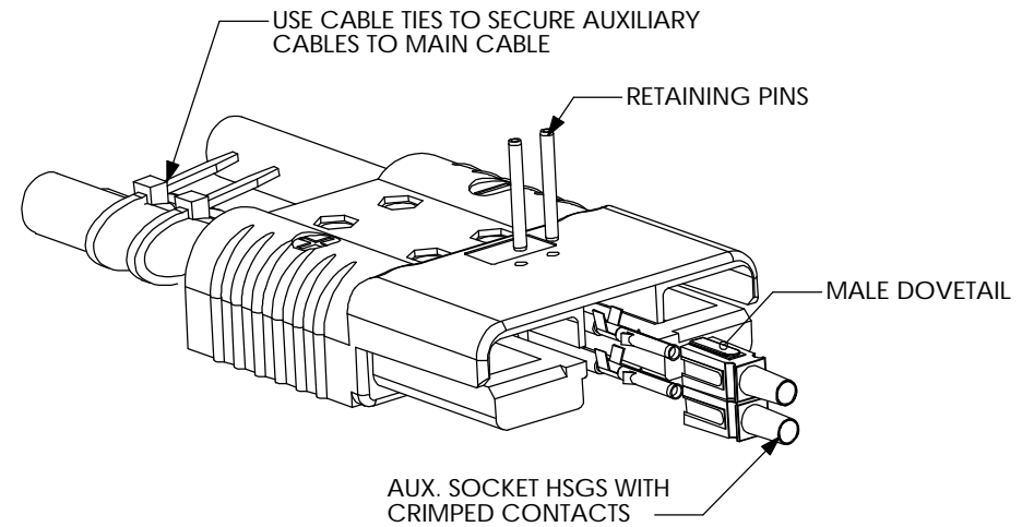
EXPLODED VIEW
